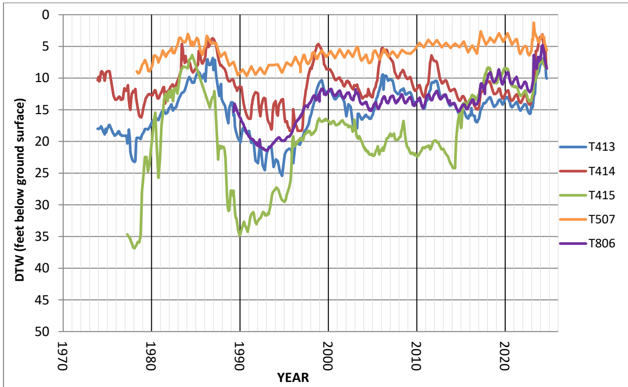
Hydrographs of selected test wells in the Thibaut-Sawmill wellfield.
