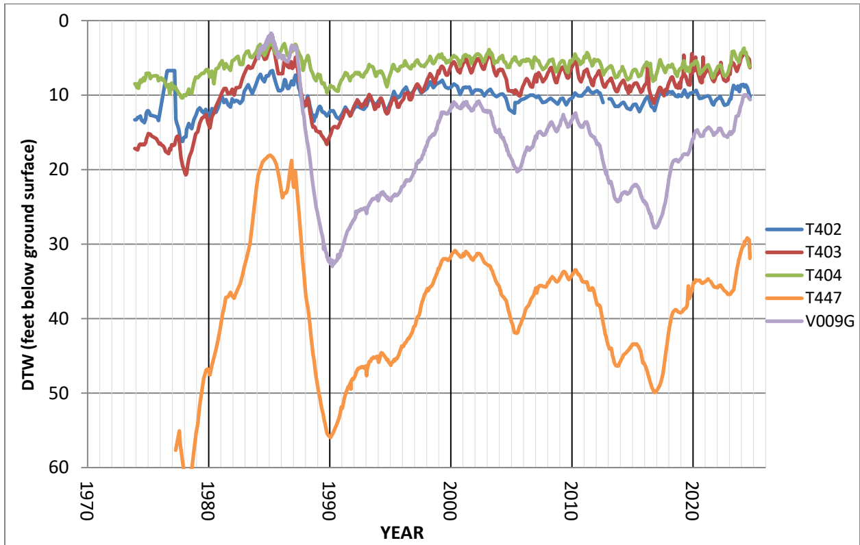
Hydrographs of Indicator wells in the Symmes-Shepherd wellfield.
