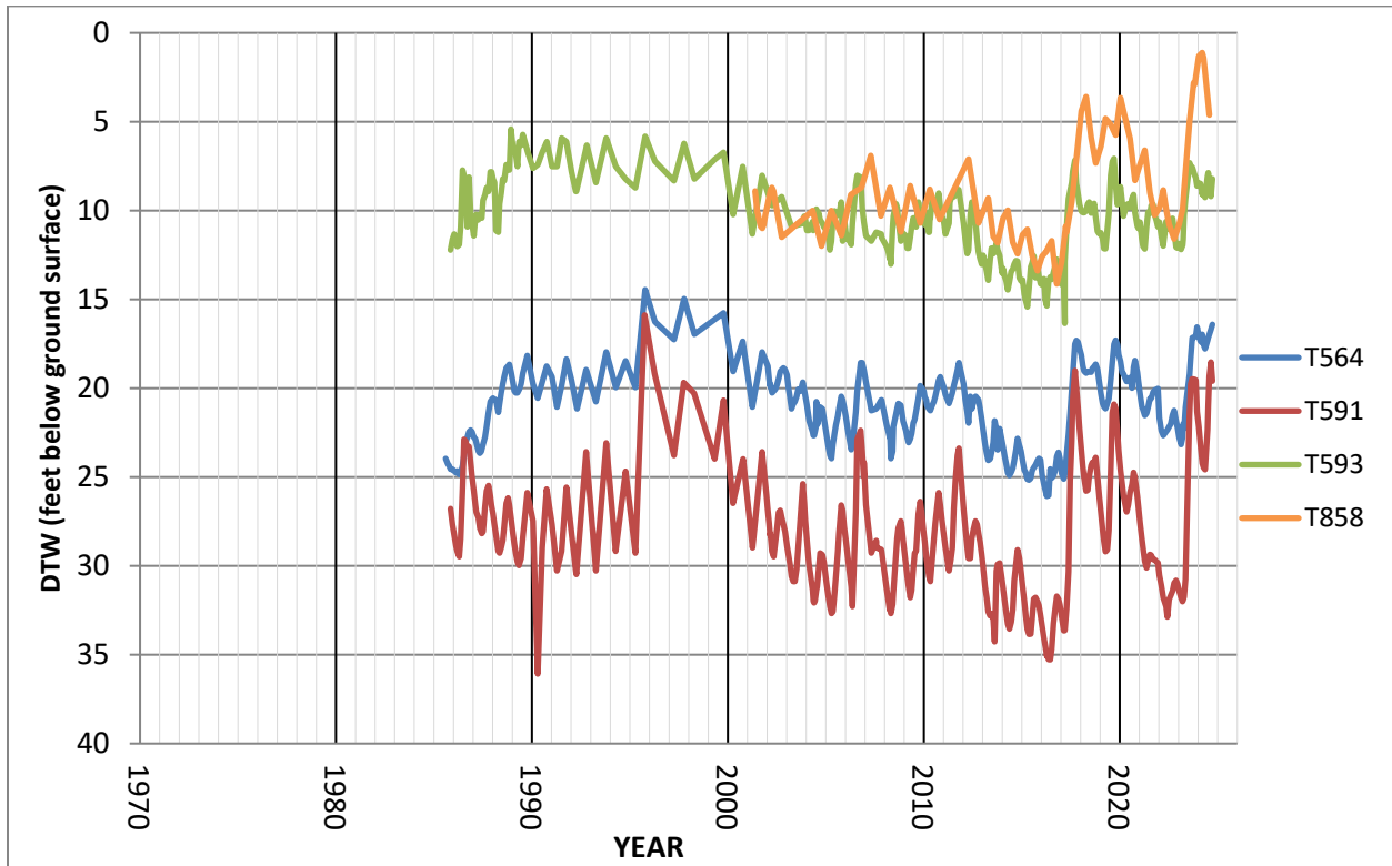
Hydrographs of selected test wells in the Lone Pine wellfield.
