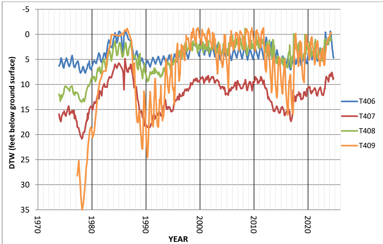
Hydrographs of selected test wells in the Independence-Oak wellfield.
