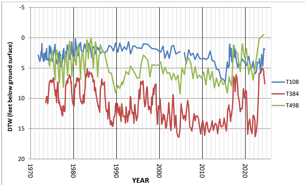
Hydrographs of selected monitoring wells in the northern Bishop wellfield.
