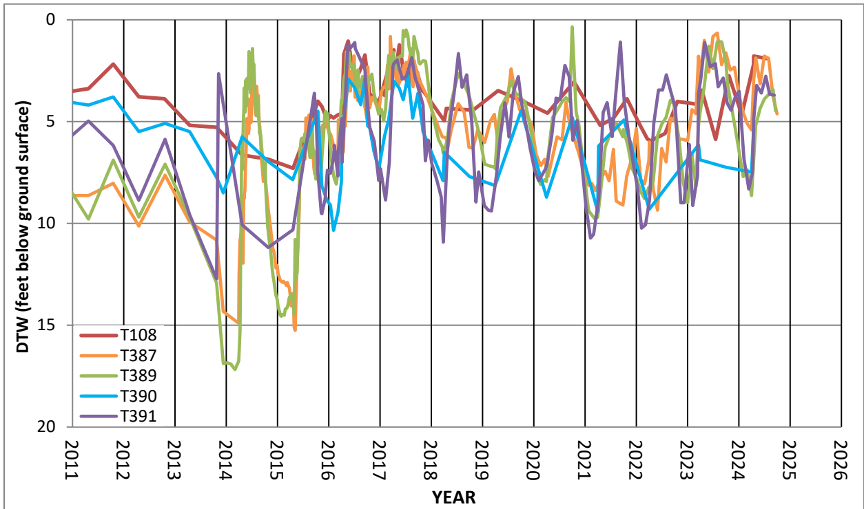
Recent hydrographs of selected monitoring wells in western Bishop wellfield.
