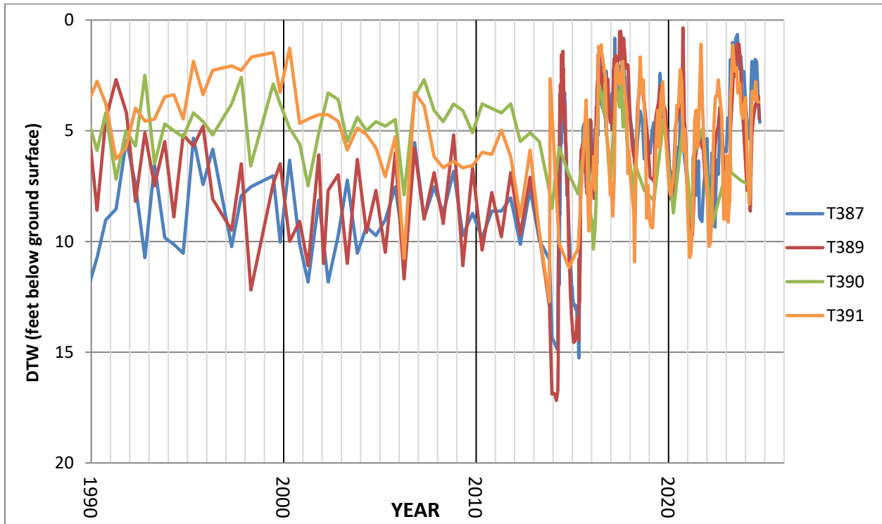
Hydrographs of selected monitoring wells in the western Bishop wellfield.
