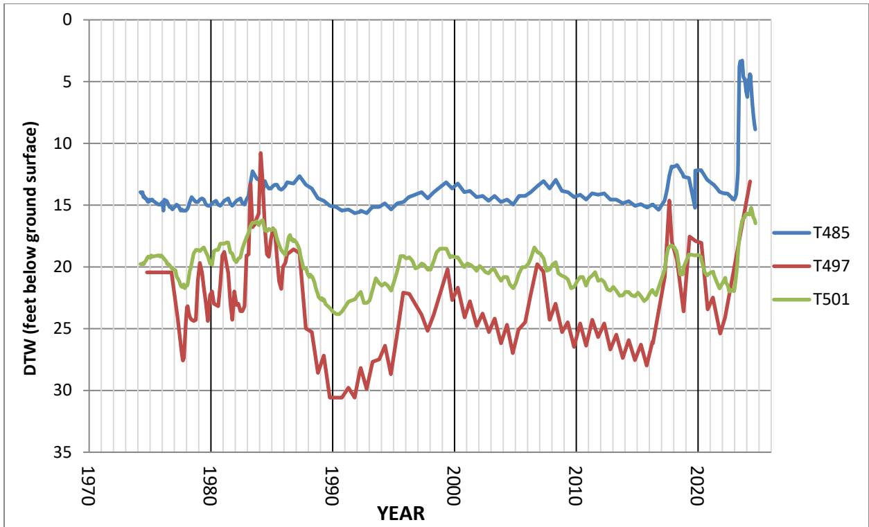
Hydrographs of selected monitoring wells in the eastern Bishop wellfield.
