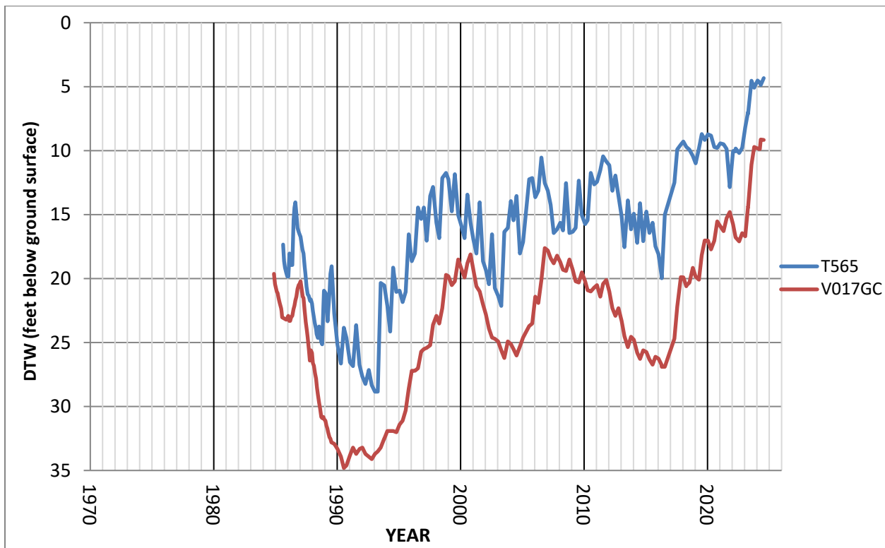
Hydrographs of monitoring wells in the southern Big Pine wellfield near pumping wells W218 and W219.
